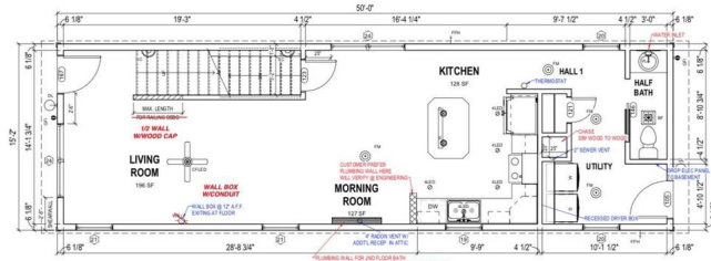
1 1ST FLOOR PLAN 01A SCALE: 1/8" = 1'-0" SCALE (TYP) 3/8" = 1'-0"
